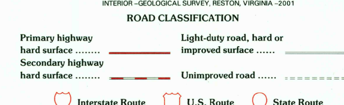
ROAD CLASSIFICATION
