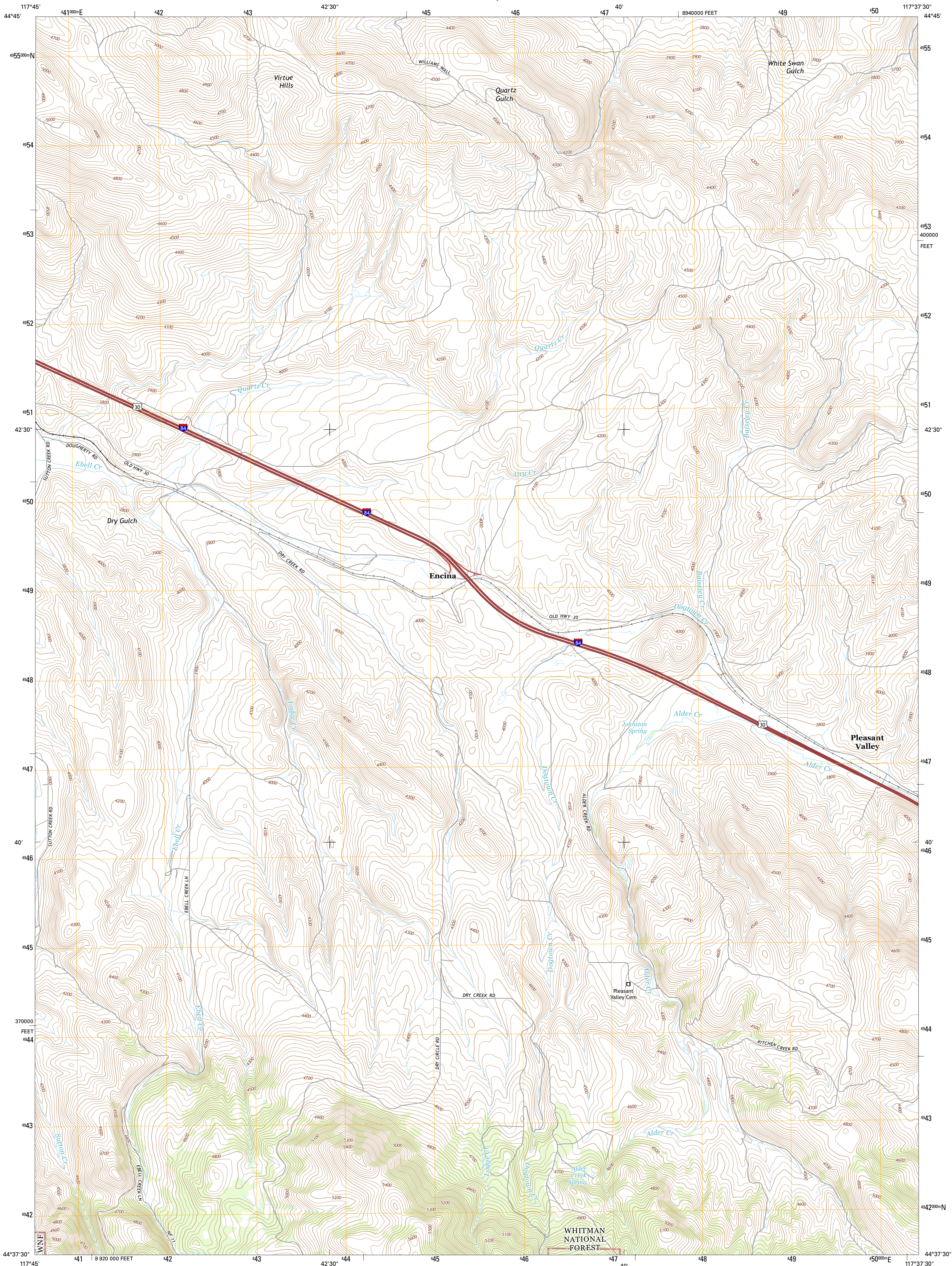
QUADRANGLE LOCATION
