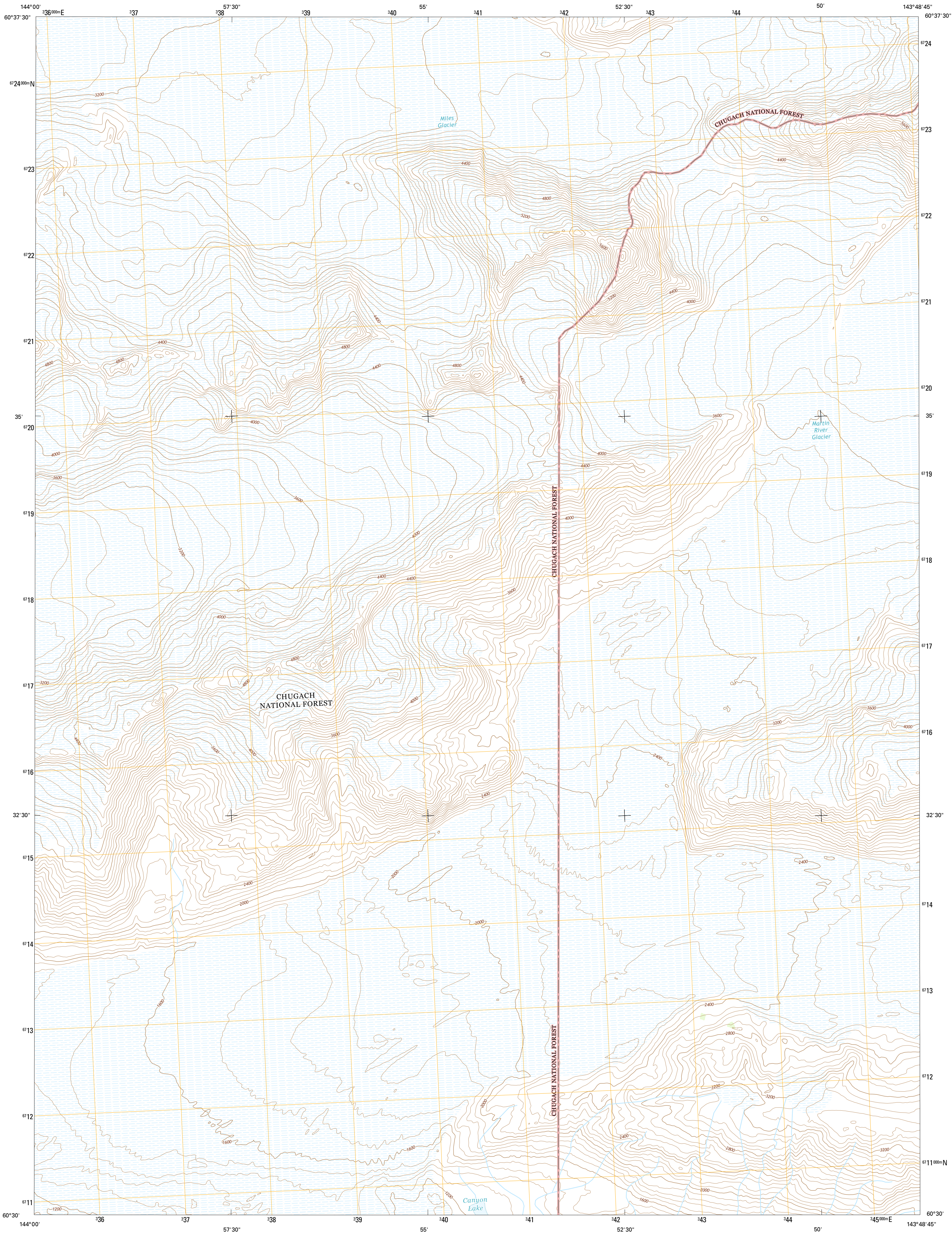
QUADRANGLE LOCATION
