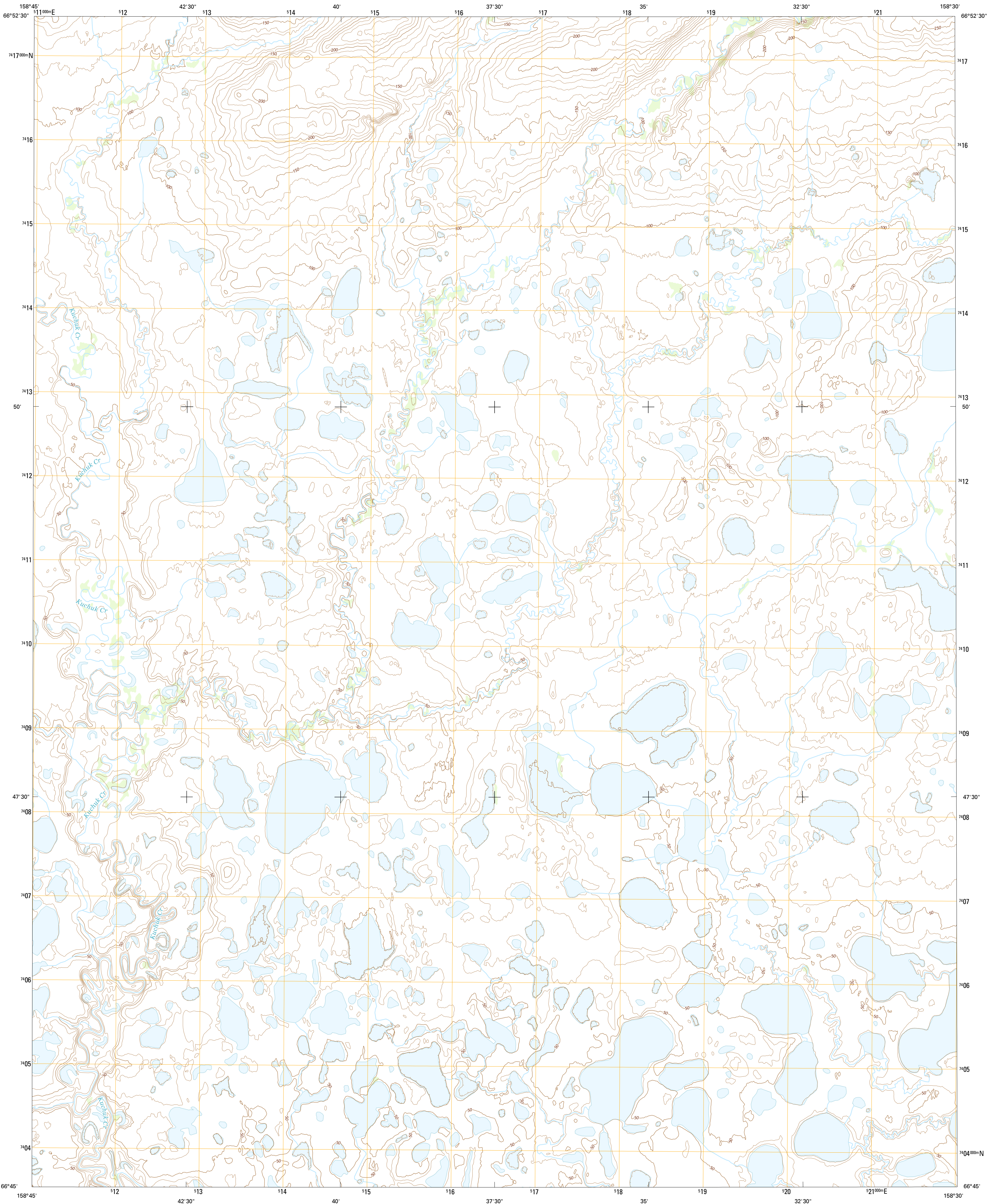
QUADRANGLE LOCATION
